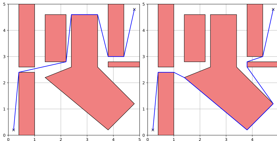
Figure 6.10 - Left : The GcsTrajOpt solution with a minimum-distance cost. Right : The GcsTrajOpt solution with a minimum-time cost (and velocity constraints).
